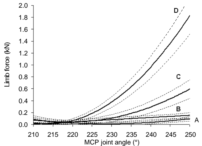
Fig 3: Mean \pm s.e. support effect for the neoprene exercise boot (A) and the Dalmar tendon support boot at resistance settings 1 (B), 2 (C) and 3 (D) ( n = 7 ).
