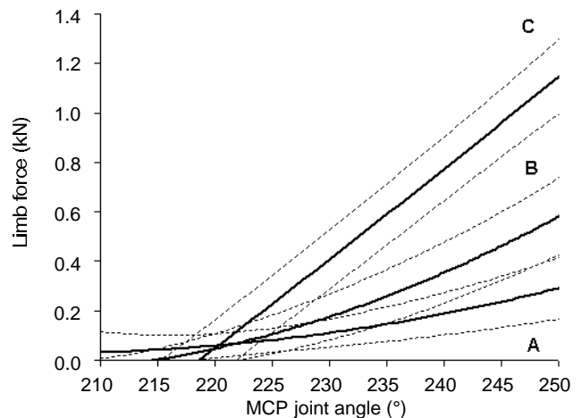
Fig 4: Mean \pm s.e. support effect for gamgee bandage (A), modified Robert Jones bandage (B) and the palmar splint (C) ( n = 7 ).
