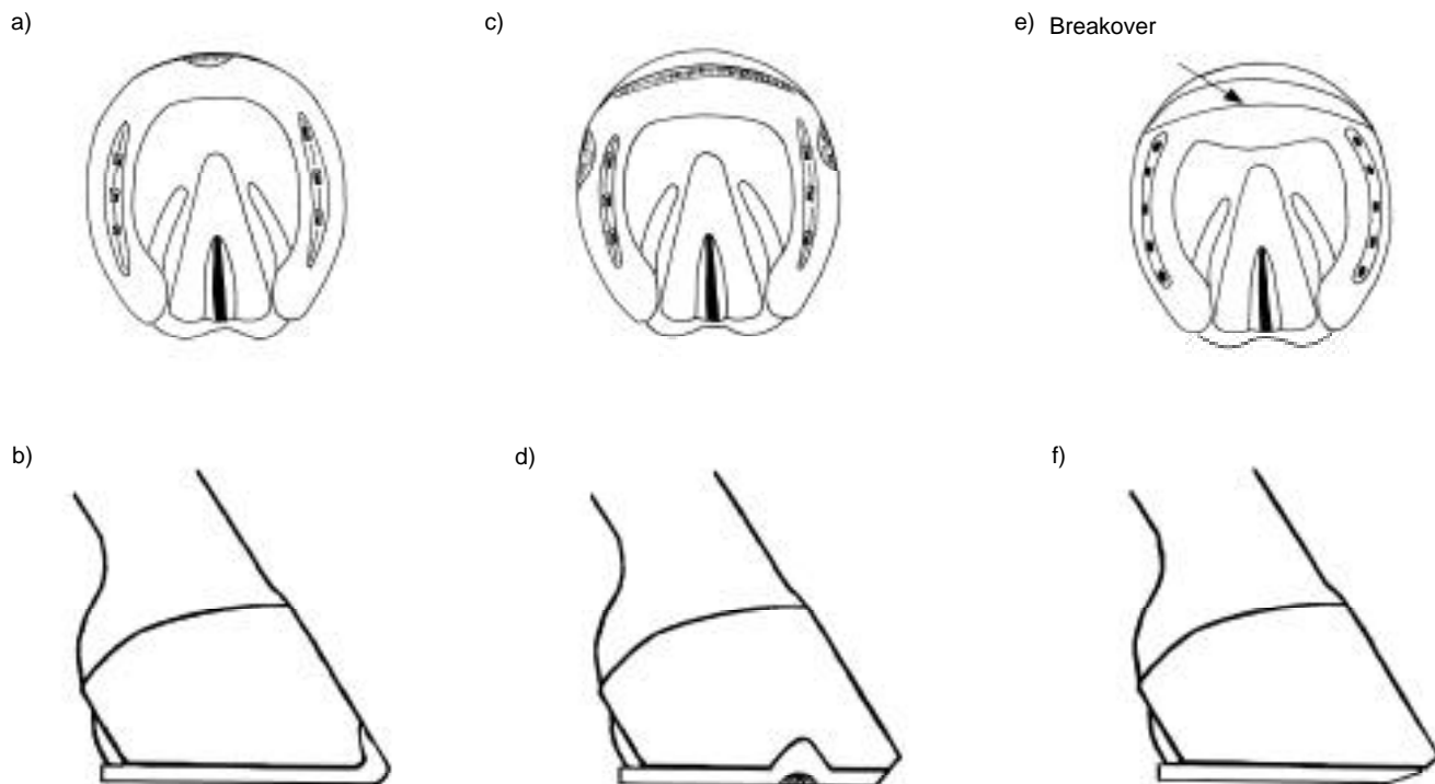
Fig 1: Solar (a) and lateromedial (b) views of the toe-clip shoe, solar (c) and lateromedial (d) views of the quarter-clip shoe and solar (e) and lateromedial (f) views of the Natural Balance shoe.
