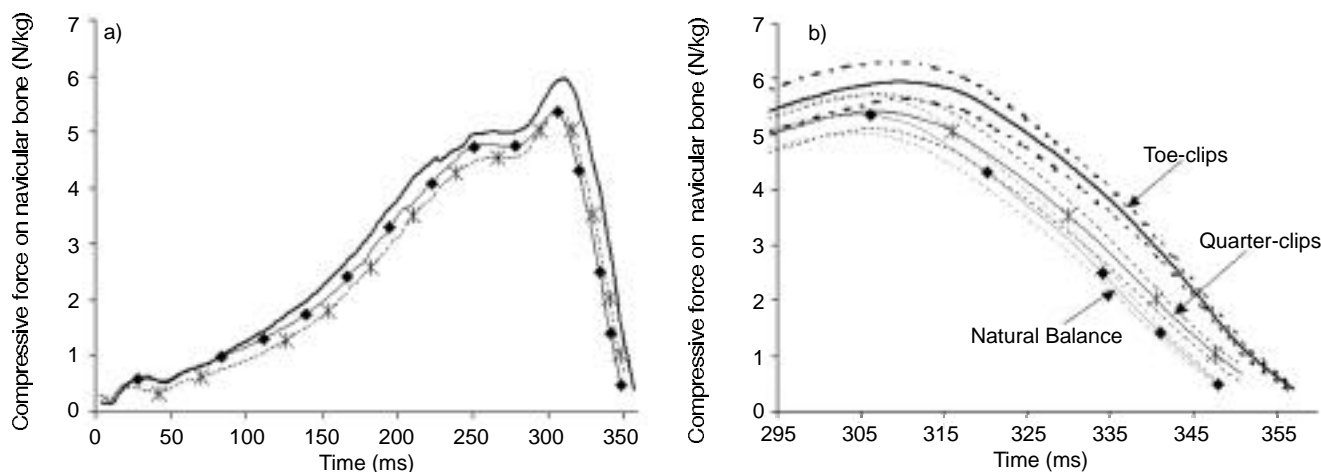
Fig 7: Graph of mean force exerted by the DDFT on the navicular bone plotted against mean stance time a) for the whole of the stance phase; b) for the end of stance. Toe clip (plain line), quarter-clip (*) and Natural Balance shoes (◆). Dotted lines represent \pm 1 s.e., n = 18 .
