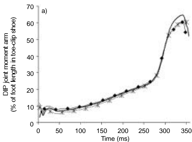
Fig 3: Graph of mean DIP joint moment arm plotted against mean stance time a) for the whole of the stance phase; b) for the end of stance. Plain line = toe-clips; * = quarter-clips; \blacklozenge = Natural Balance. Dotted lines represent \pm 1 s.e., n = 18 .
