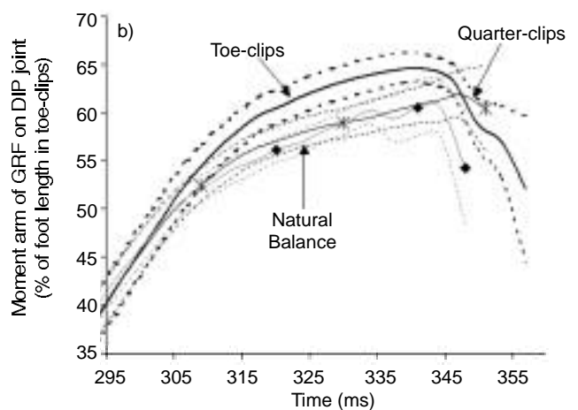
Fig 3: Graph of mean DIP joint moment arm plotted against mean stance time a) for the whole of the stance phase; b) for the end of stance. Plain line = toe-clips; * = quarter-clips; \blacklozenge = Natural Balance. Dotted lines represent \pm 1 s.e., n = 18 .
